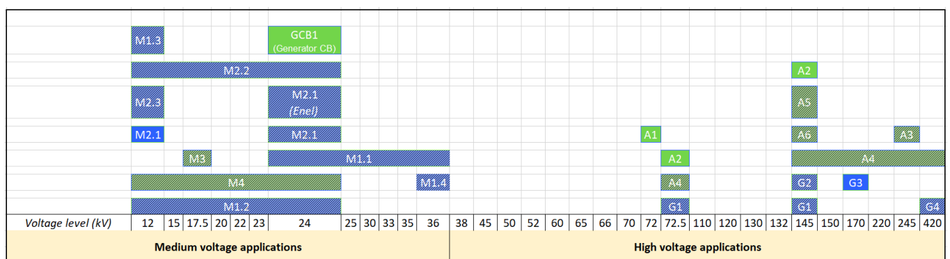
Chart 1: Currently available SF 6 -free equipment for MV and HV applications
